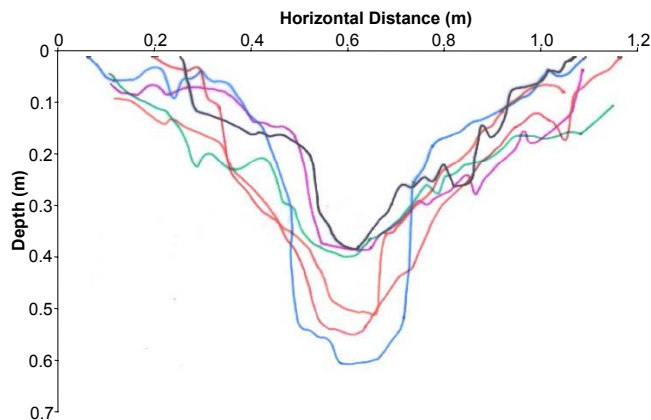
Figure 2: Breakout profiles using a no-wing subsoiler tine in clay restored soil.
