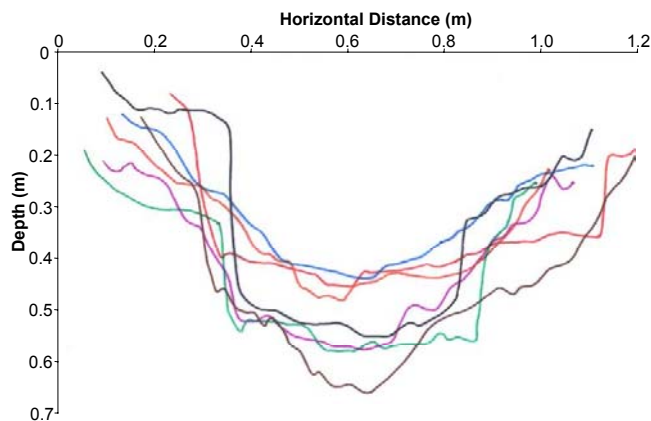
Figure 3: Breakout profiles using a high-lift height winged subsoiler tine in clay restored soil.
