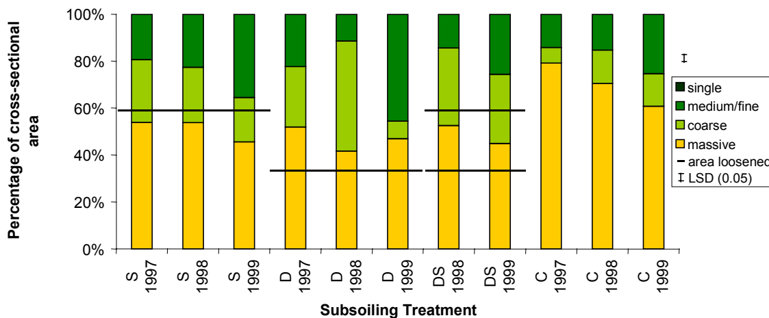
Figure 7: Effect of loosening on soil structural zones at Wollaston Sand.
