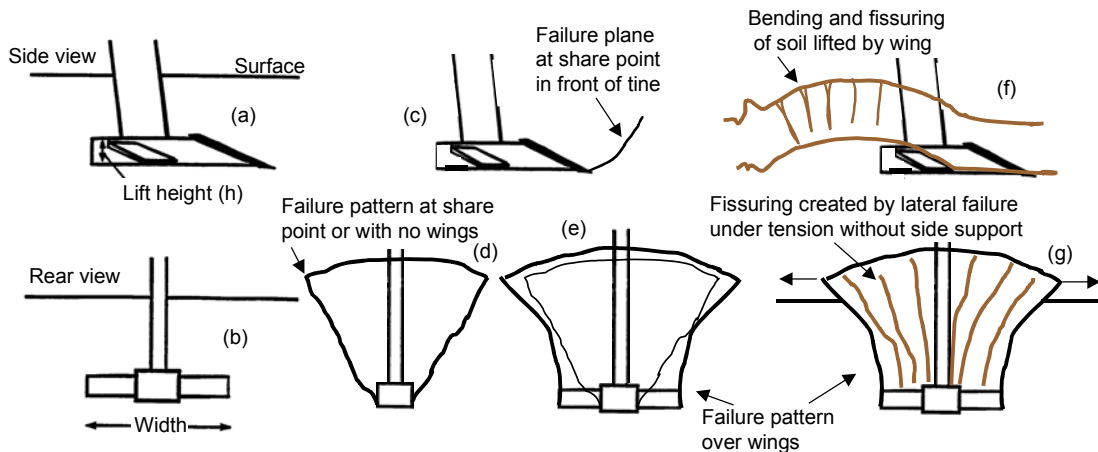
Figure 1: Influence of tine geometry on observed soil profile disturbance.
